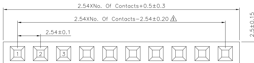
Recommended P.C.B. Layout(Top View) (PCB Board Tolerance±0.05)
