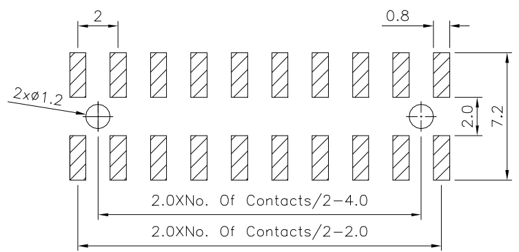
Recommend P.C.B Board Layout PCB Tolerance:±0.05(Top View)
