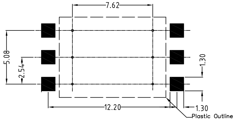
(.XX ±0.05 For PCB) Reference PCB Layout
