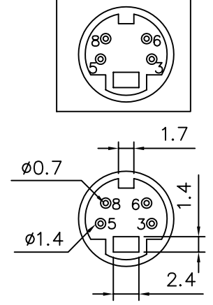
Arrangement Of Contacts
