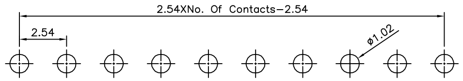
Recommended P.C.B. Layout(Top View) (PCB Board Tolerance±0.05)
