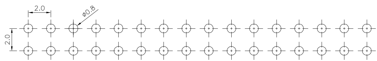
Recommended P.C.B. Layout
