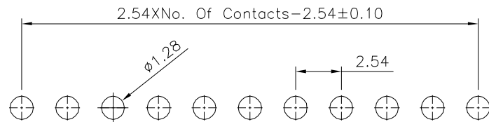
Recommended P.C.B Layout Tolerance±0.05
