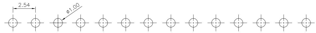
Recommended P.C.B. Layout △ Tolerance ±0.05
