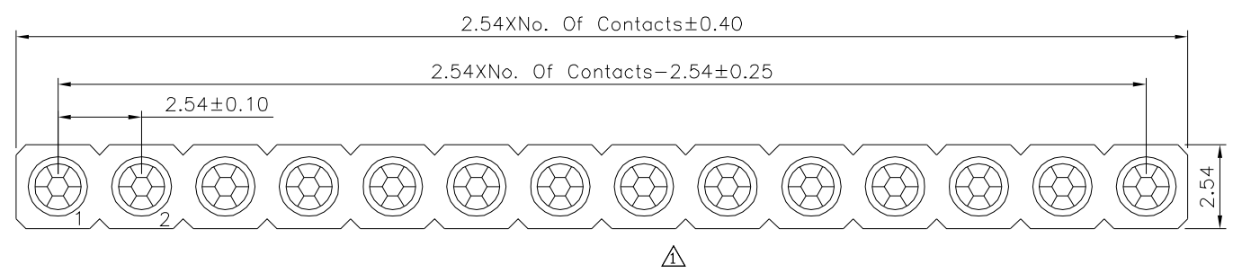
Recommended P.C.B. Layout △ Tolerance ±0.05
