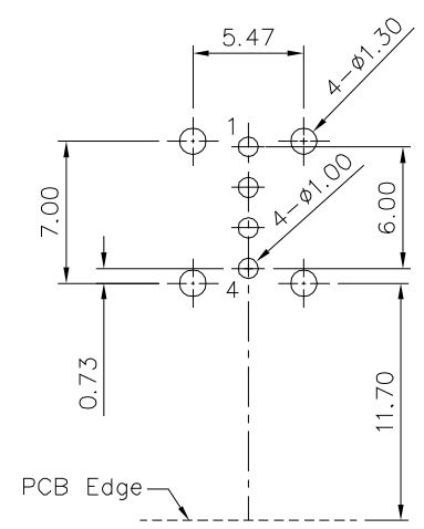
Recommended P.C.B. Layout(Top View) PCB Thickness:1.60±0.05,Tolerance±0.05
