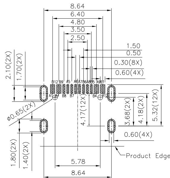
Recommended P.C.B. Layout(Top View) Thickness 0.80mm,Tolerance:±0.05
