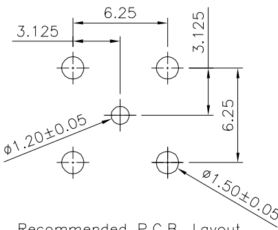
Recommended P.C.B. Layout Without Mounting Posts
