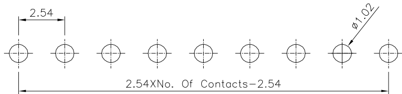
Recommended P.C.B. Layout(Top View) (PCB Board Tolerance±0.05)
