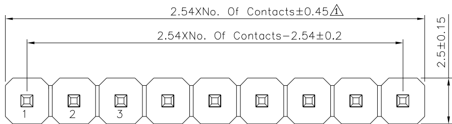
Recommended P.C.B. Layout(Top View) (PCB Board Tolerance±0.05)
