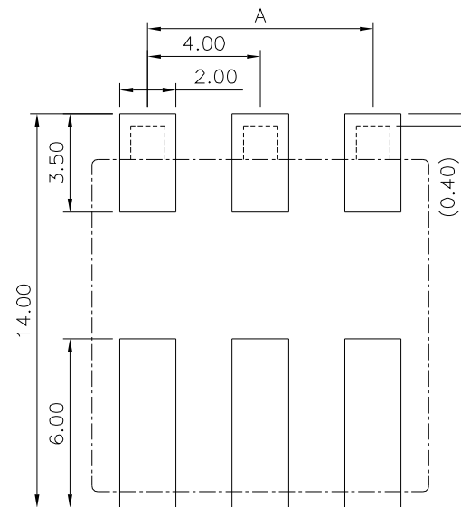
Recommended P.C.B. Layout Tolerance: ±0.05 (Top View)
