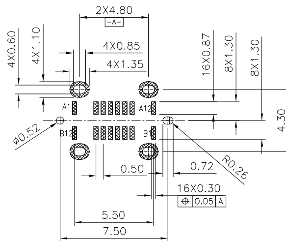
Recommended P.C.B. Layout(Top View) Thickness:0.8±0.10(Tolerance±0.05)
