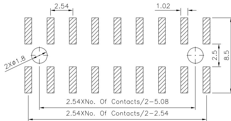
Recommended P.C.B. Layout(Top View) (PCB Board Tolerance \pm 0.05 )
