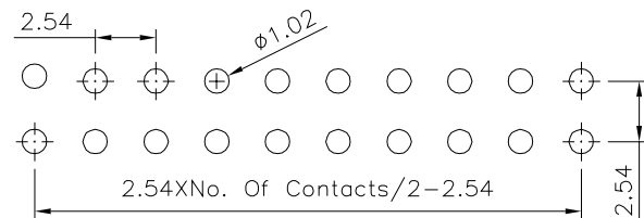
Recommended P.C.B. Layout(Top View) (PCB Board Tolerance±0.05)
