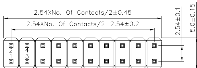
Recommended P.C.B. Layout(Top View) (PCB Board Tolerance±0.05)
