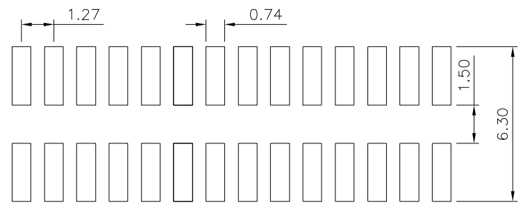
Recommended P.C.B. Layout (PCB Board Tolerance±0.05)
