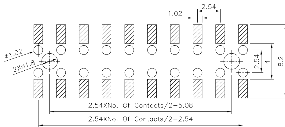
Recommended P.C.B. Layout(Top View) (PCB Board Tolerance±0.05)
