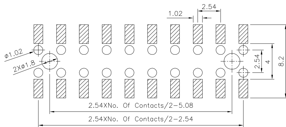
Recommended P.C.B. Layout(Top View) (PCB Board Tolerance±0.05)
