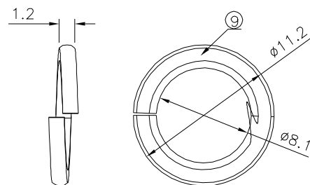
Gap Washer
