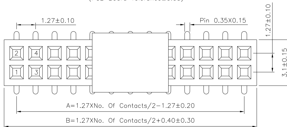
Recommended P.C.B. Layout (PCB Board Tolerance±0.05)
