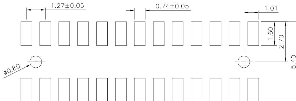
Recommended P.C.B. Layout (PCB Board Tolerance±0.05)
