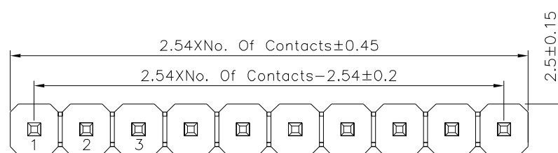
Recommended P.C.B. Layout(Top View) (PCB Board Tolerance±0.05)
