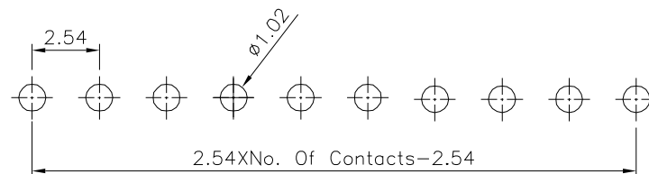
Recommended P.C.B. Layout(Top View) (PCB Board Tolerance±0.05)
