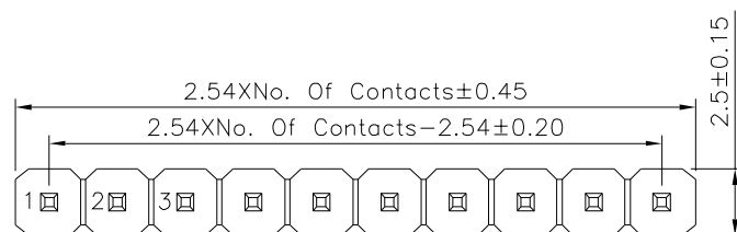
Recommended P.C.B. Layout(Top View) (PCB Board Tolerance±0.05)
