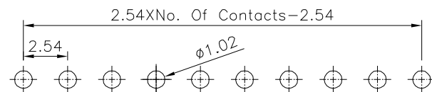
Recommended P.C.B. Layout(Top View) (PCB Board Tolerance±0.05)
