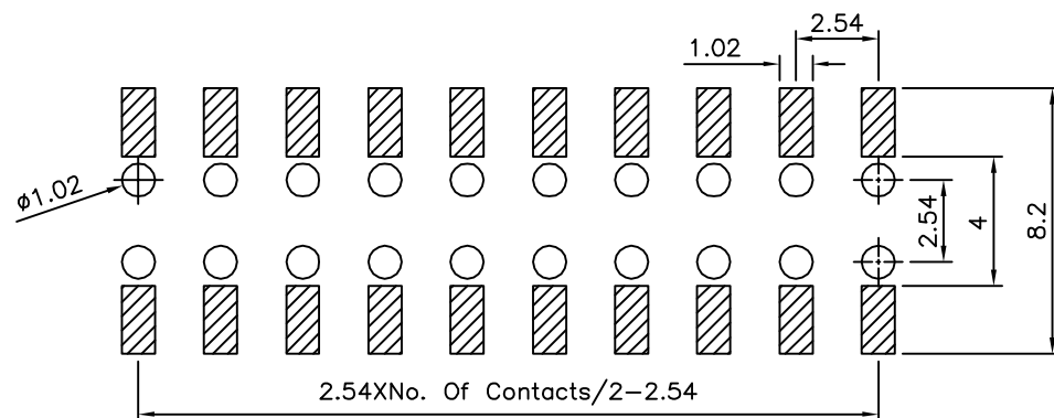
Recommended P.C.B. Layout(Top View) (PCB Board Tolerance±0.05)
