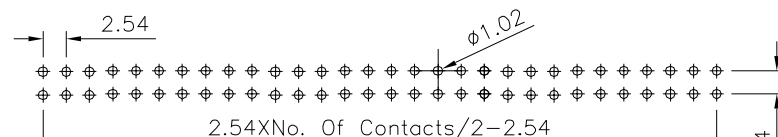
Recommended P.C.B. Layout(Top View) (PCB Board Tolerance±0.05)
