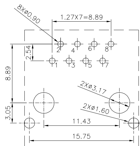
△ P.C.B. Layout Component Side Tolerances±0.05(Thickness=1.6mm)
