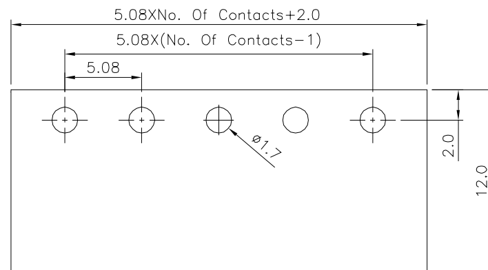
① Recommended P.C.B. Layout
