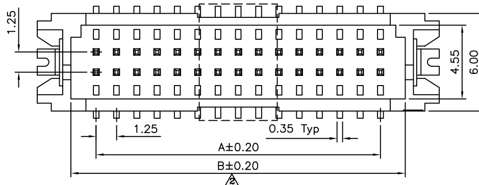
Recommended P.C.B. Layout(Top Side) (PCB Board Tolerance±0.05) △
