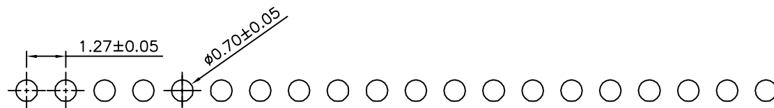
Recommended P.C.B. Layout
