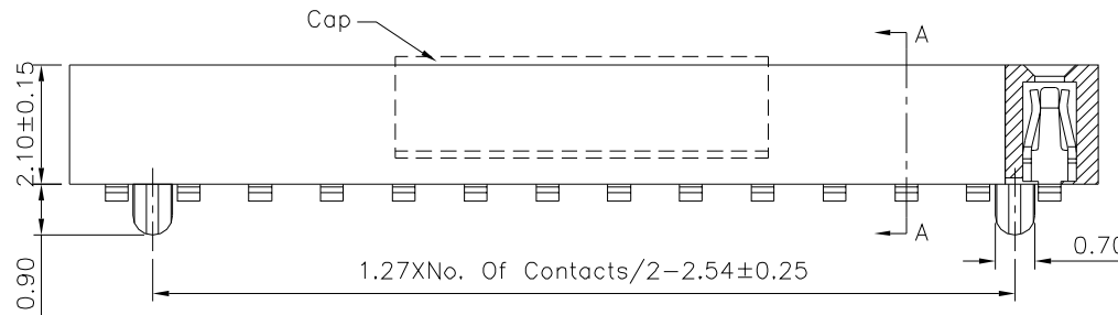
Section B-B
