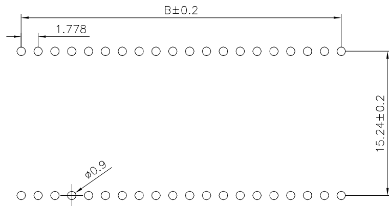
1 Recommended P.C.B. Layout
