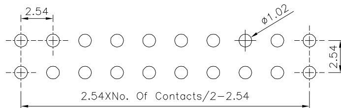
Recommended P.C.B. Layout(Top View) (PCB Board Tolerance±0.05)
