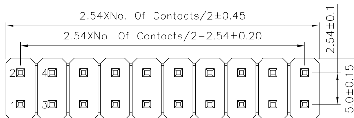
Recommended P.C.B. Layout(Top View) (PCB Board Tolerance±0.05)
