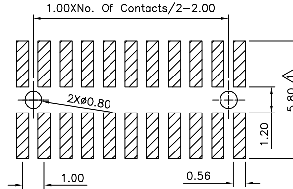
Recommended P.C.B. Layout(Top Side) (PCB Board Tolerance±0.05)
