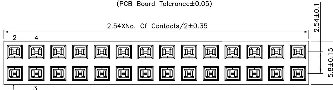
Recommended P.C.B. Layout(Top View) (PCB Board Tolerance±0.05)
