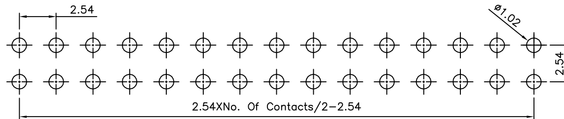
Recommended P.C.B. Layout(Top View) (PCB Board Tolerance±0.05)
