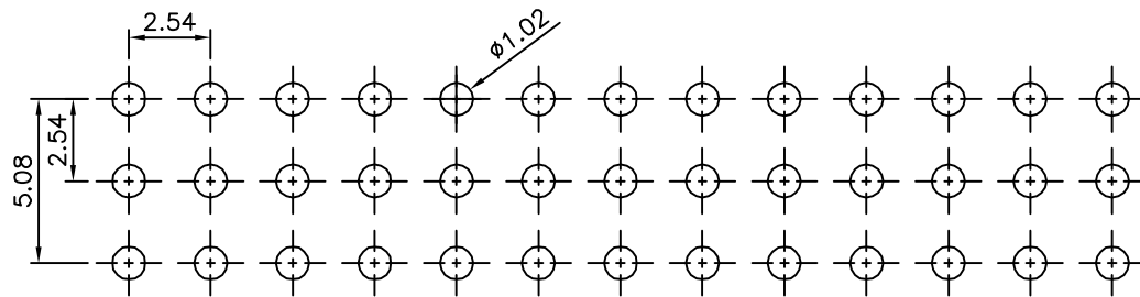
Recommended P.C.B. Layout(Top Side) (PCB Board Tolerance \pm 0.05 )
