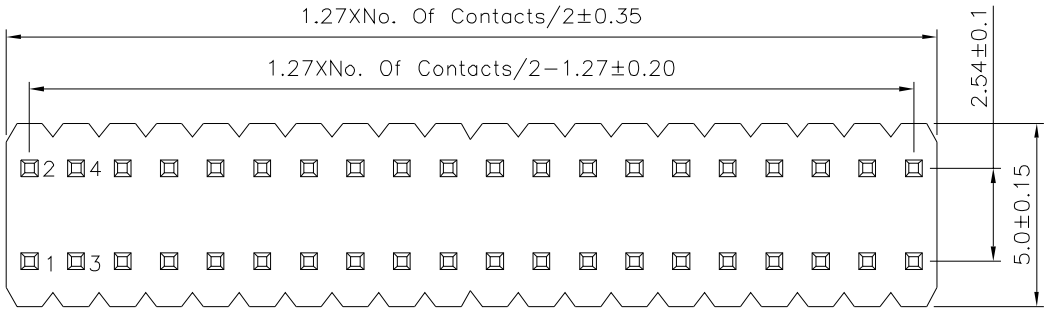
Recommended P.C.B. Layout(Top View) (PCB Board Tolerance±0.05)
