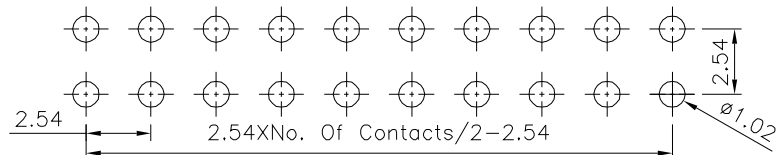
Recommended P.C.B. Layout(Top View) (PCB Board Tolerance±0.05)
