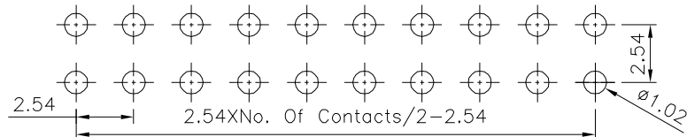
Recommended P.C.B. Layout(Top View) (PCB Board Tolerance \pm 0.05 )
