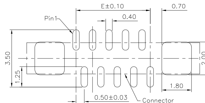
4/3 Recommended PCB Layout
