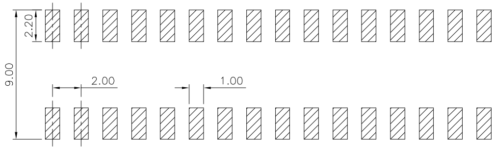
Recommended P.C.B. Layout(Top Side) (PCB Board Tolerance±0.05)
