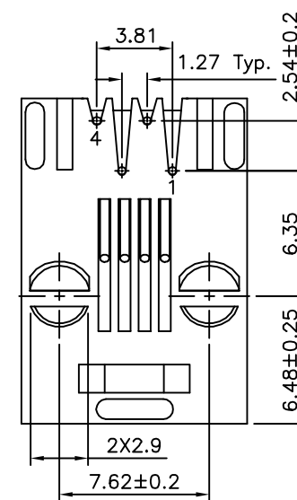
Recommended P.C.B. Layout(Top View) PCB Thickness:1.6mm Tolerance:±0.05
