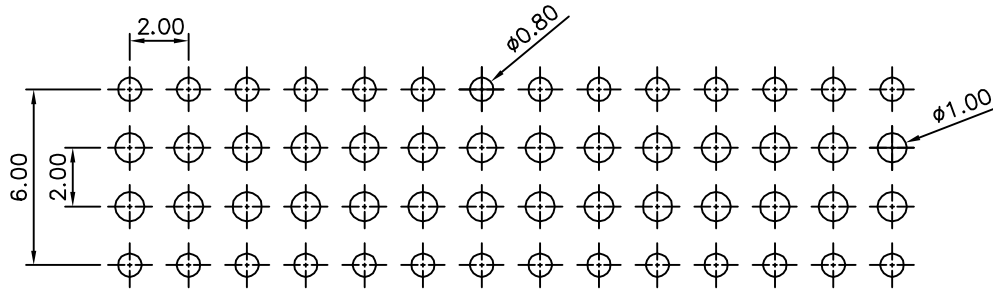
Recommended P.C.B. Layout(Top Side) (PCB Board Tolerance±0.05)
