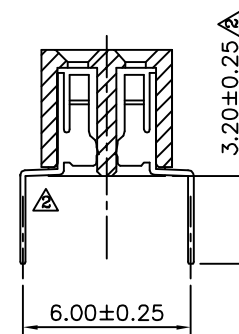
Section L-L
