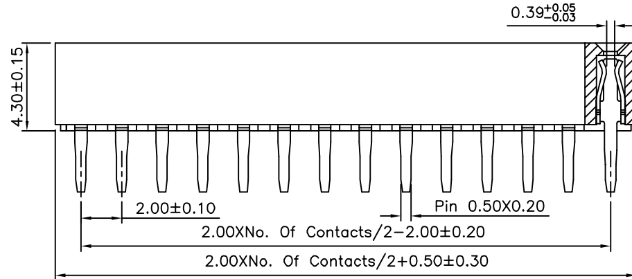
Section B-B
