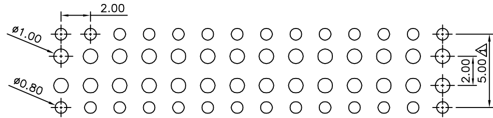
Recommended P.C.B. Layout(Top Side) (PCB Board Tolerance \pm 0.05 )
