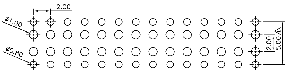
Recommended P.C.B. Layout(Top Side) (PCB Board Tolerance±0.05)
