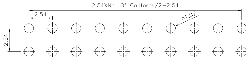
Recommended P.C.B. Layout(Top View) (PCB Board Tolerance±0.05)
