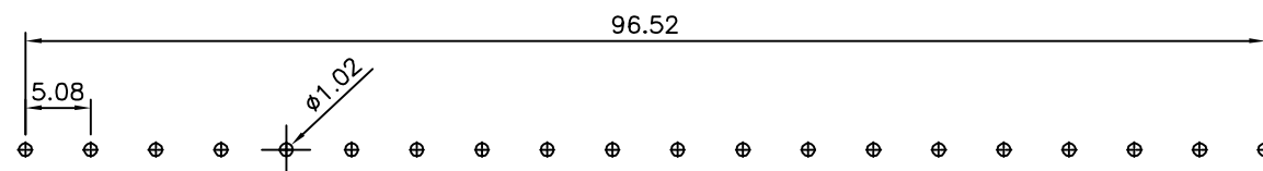
Recommended P.C.B. Layout(Top View) (PCB Board Tolerance±0.05)
