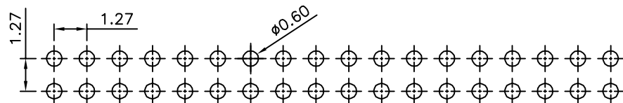
Recommended P.C.B. Layout(Top Side) (PCB Board Tolerance±0.05)
