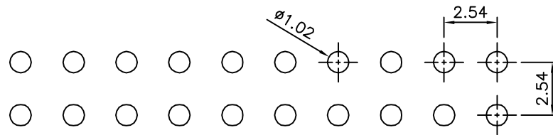
Recommended P.C.B. Layout(Top Side) (PCB Board Tolerance \pm 0.05 )
