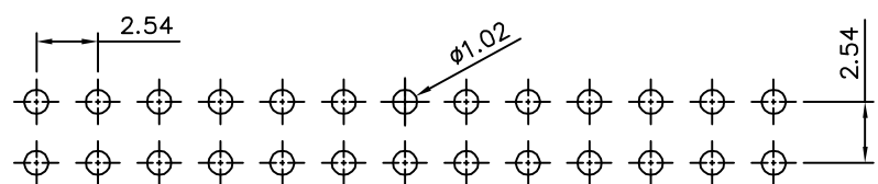
Recommended P.C.B. Layout(Top Side) (PCB Board Tolerance±0.05)
